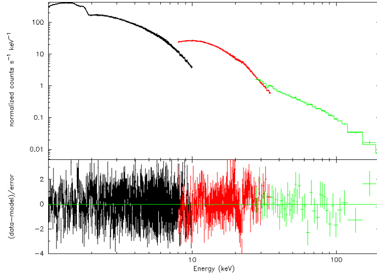
Fig. 4-31 Spectra of Crab nebula observed by Insight -HXMT in 982 s.
