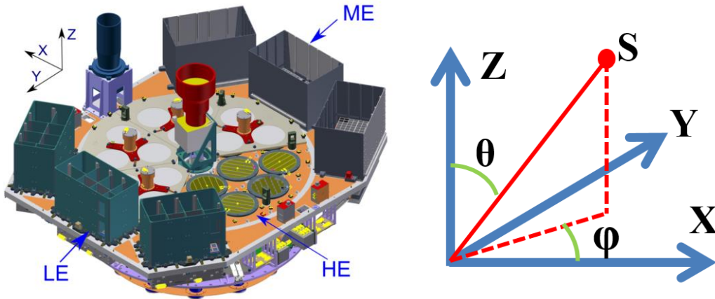
Fig. 3-9 (Left) Definition of the payload coordinate. (Right) Illustration of the incident angle (zenith angle \theta and azimuthal angle \phi ) of gamma-ray sources (S) in the payload coordinate.
