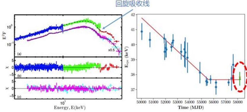
Fig. 4-36 Insight -HXMT confirms that the long-term decaying trend of the Her X-1 CRSF centroid energy has stopped (Xiao et al. 2019).
