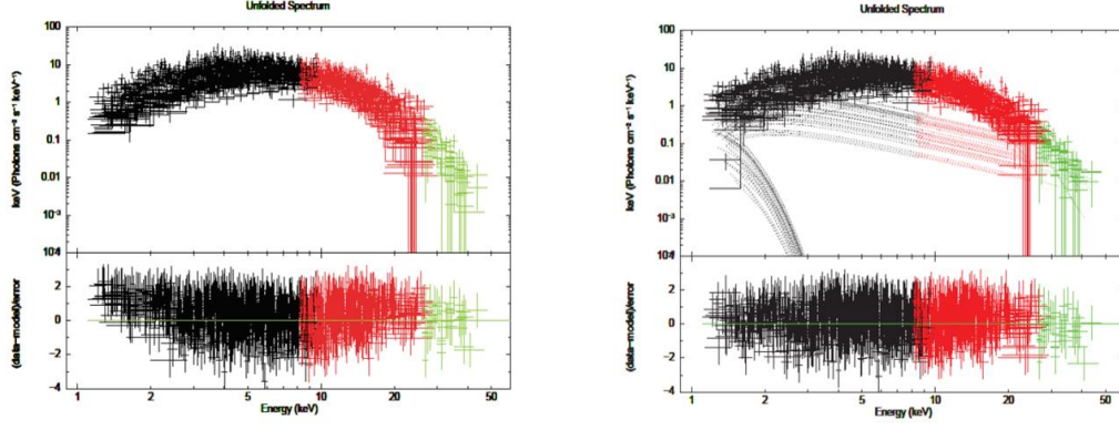
Fig. 4-39 the merged spectra fitted with an absorbed black-body model (left) and the f_a model (right). The dotted lines represent the model components for the pre-burst emission (blackbody and nthcomp ). (Chen et al. 2019)
