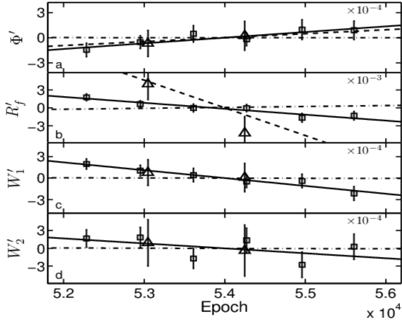
Fig. 4-9 Evolution of pulse shape of Crab observed by RXTE. The square and triangle are the results from PCA and HEXTE, respectively. From upward to downward the panels are: peak separation, flux ratio, width of main peak and the second peak. All data are deduced their mean value. The solid line is the linear fitting result, dot line is the fitting result of response phase of
