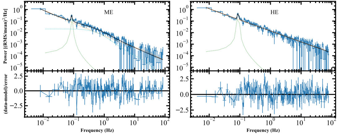
Fig 4-26 A new type of LFQPO detected in the soft state of Cygnus X-1 (Yan et al. 2021)
