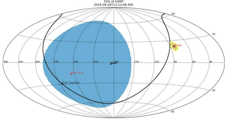
Fig. 3-12 the FOV of Insight -HXMT as a gamma-ray all-sky monitor at 2019-09-28T13:13:48.400. The blue region represents the occulted sky by the Earth that changes with time, while the yellow region is the FOV of HE collimator.
