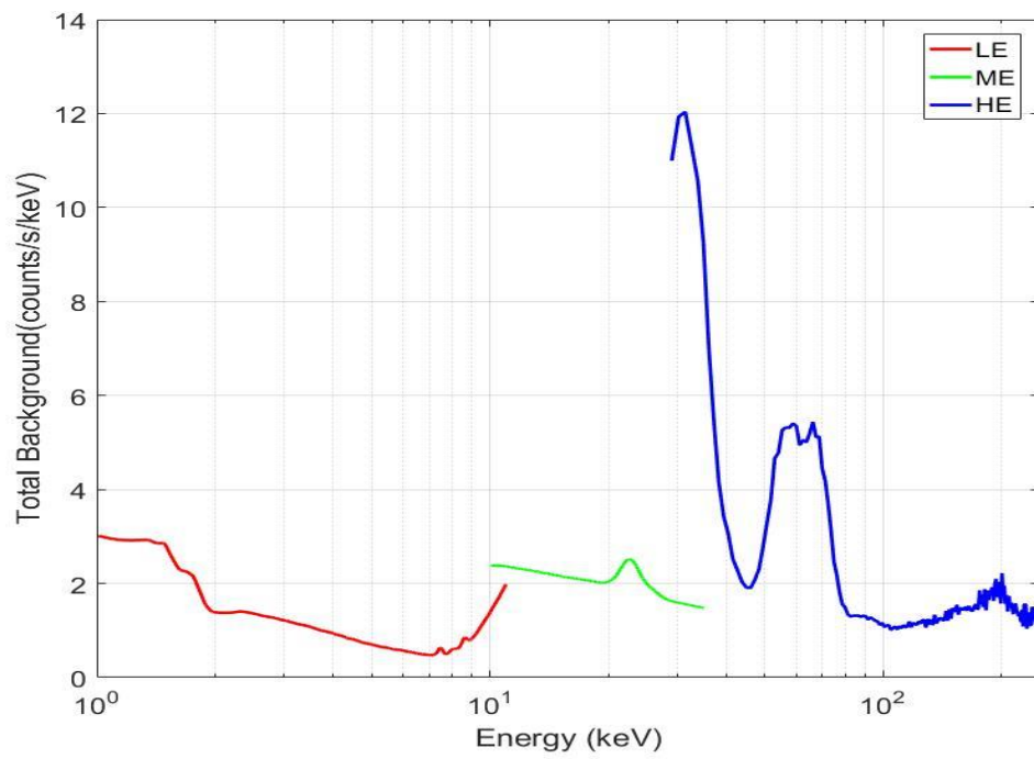
Fig. 3-33 the background spectrum of Insight-HXMT detectors.
