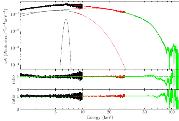
Fig. 4-35 CRSF around 90 keV detected in GRO J1008–57 with Insight -HXMT (Ge et al. 2020b).
