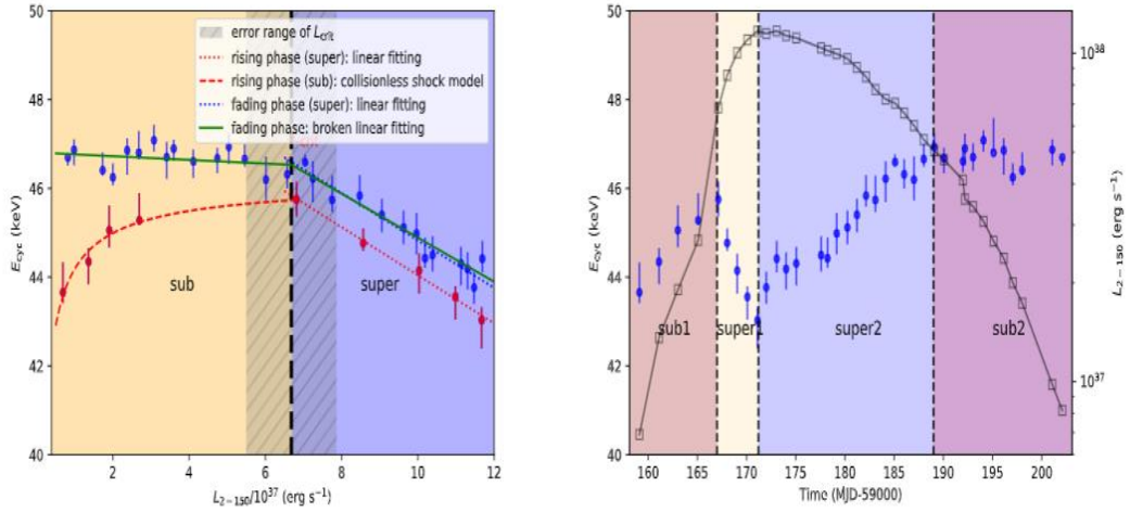
Fig. 4-37 Left panel: relation between energy of CRSF and luminosity. Right panel: evolution of energy of CRSF with time.
