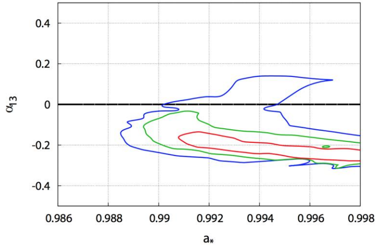
Fig 4-27 Spin measurement of MAXI J1535-571 (Q. Liu et al. 2021)
