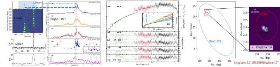
Fig. 4-41 Multiwavelength observations of Insight-HXMT and other telescopes for FRB 200428, which identified that the FRB originates from the magnetar SGR J1935+2154 (Li et al. 2021).
