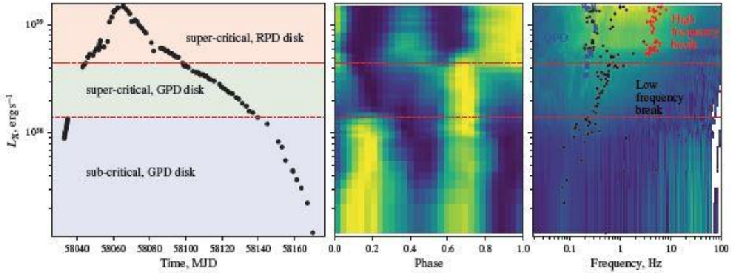
Fig. 4-28 The outburst evolution of the Galactic ULX Swift J0243.6+6124 monitored by Insight -HXMT (Doroshenko et al. 2020).
