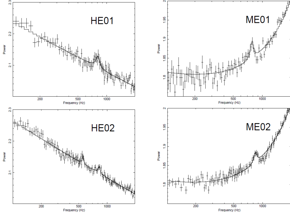
Fig. 4-40 High energy kHz QPOs in Sco X-1 observed with Insight -HXMT (Jia et al. 2020).
