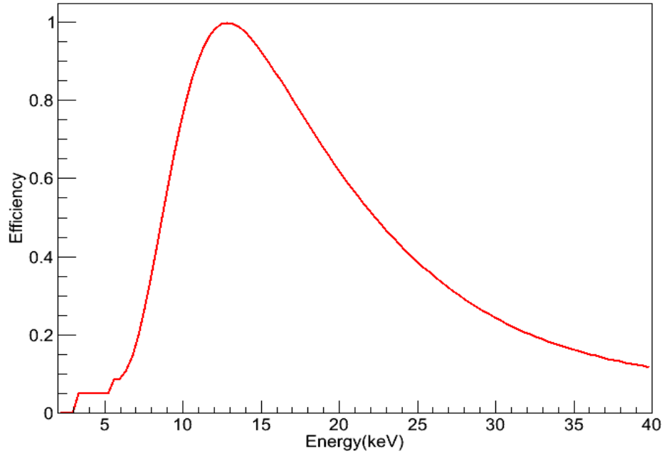
Fig. 3-22 the detection efficiency of Insight -HXMT/ME. The duty-cycle of the collimator is considered, and the area of the collimator is smaller than 850 cm 2 .
