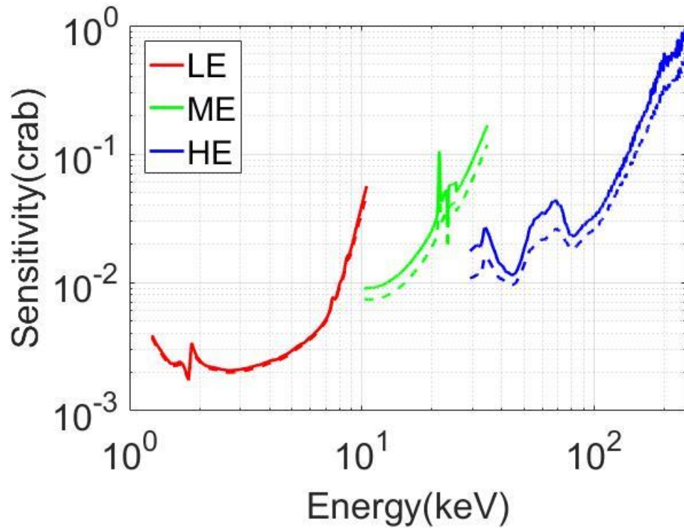
Fig. 3-34 Sensitivity of pointing observations of the three InSight -HXMT detectors (100 s, 3\sigma ).
