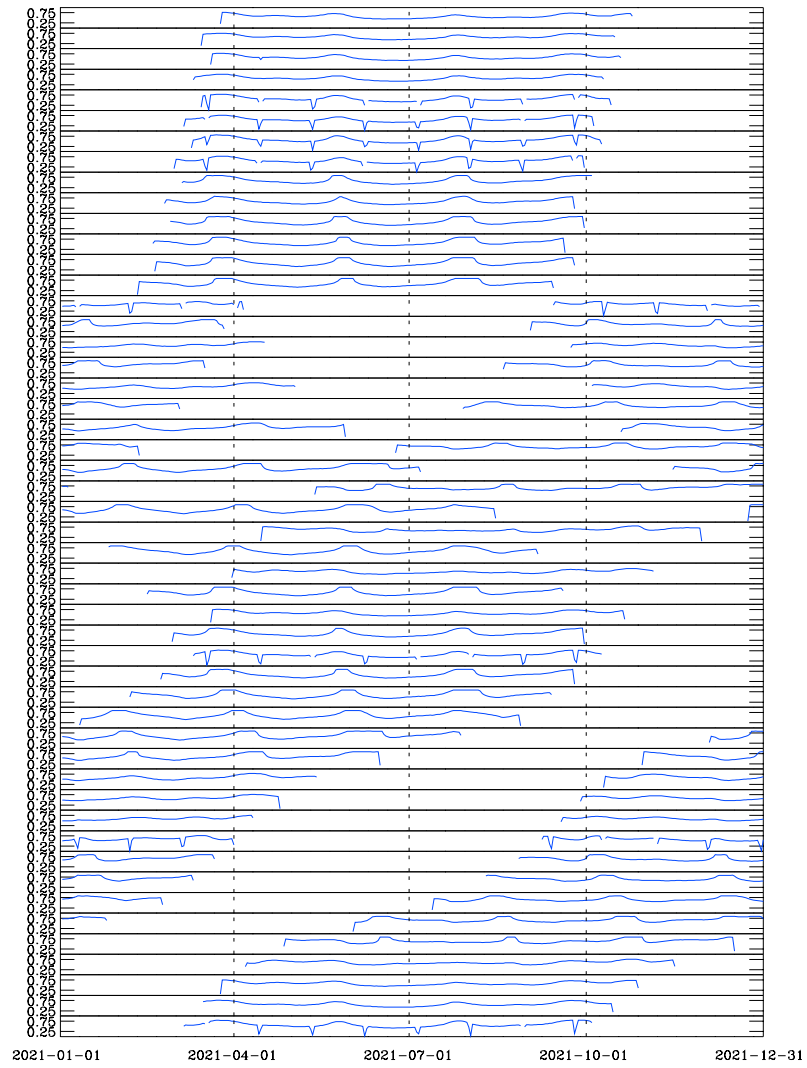
Fig. 4-1 visibility and visible efficiency of 50 observed zones
