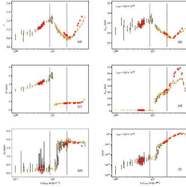
Fig.4-29 Spectral evolution of the Galactic ULX Swift J0243.6+6124 monitored by Insight-HXMT (Kong et al. 2020b)
