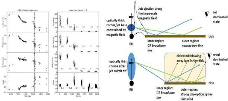
Fig 4-22 Transition from a jet-dominated state to a wind-dominated state for the flare in GRS 1915+105 (Kong et al. 2021)
