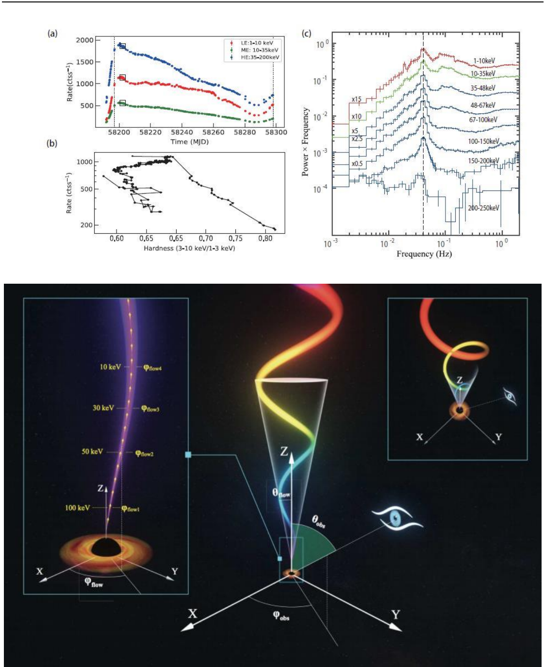
Fig. 4-18 the highest energy QPO discovered in MAXI J1820+070 (upper panel) and the model interpretation in a jet precession scenario (lower panel) (Ma et al. 2021).
