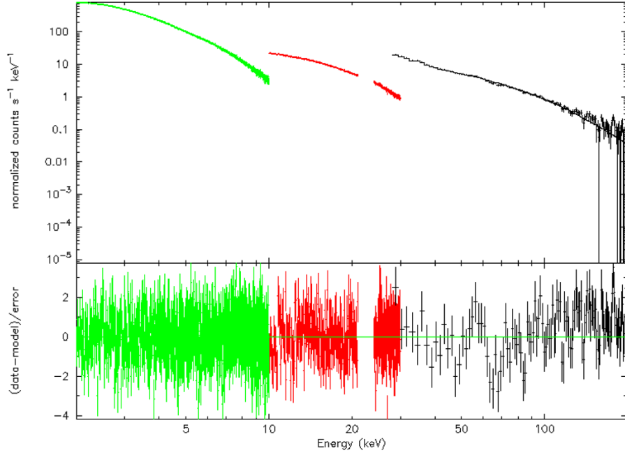
Fig. 4-34 Insight -HXMT spectra of MAXI J1820+070 in the low/hard state.
