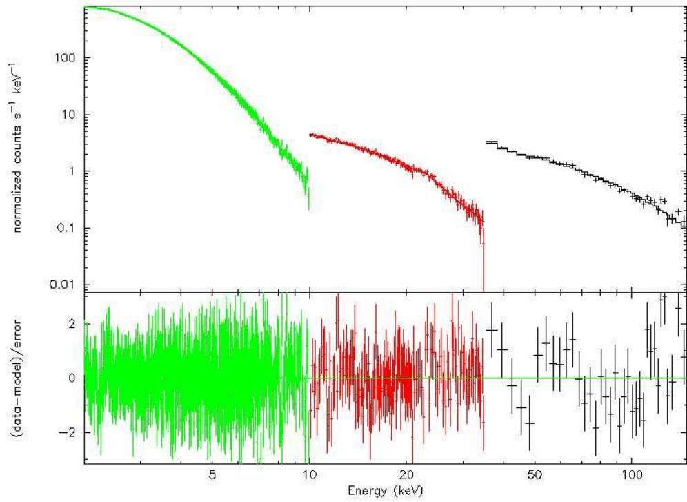
Fig. 4-33 Insight-HXMT spectra of MAXI J1820+70 in the high/soft state.
