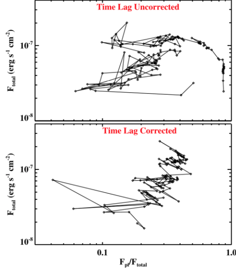
Fig 4-24 Explanation of the hysteresis effect and the "q"-diagram (Weng et al. 2021)
