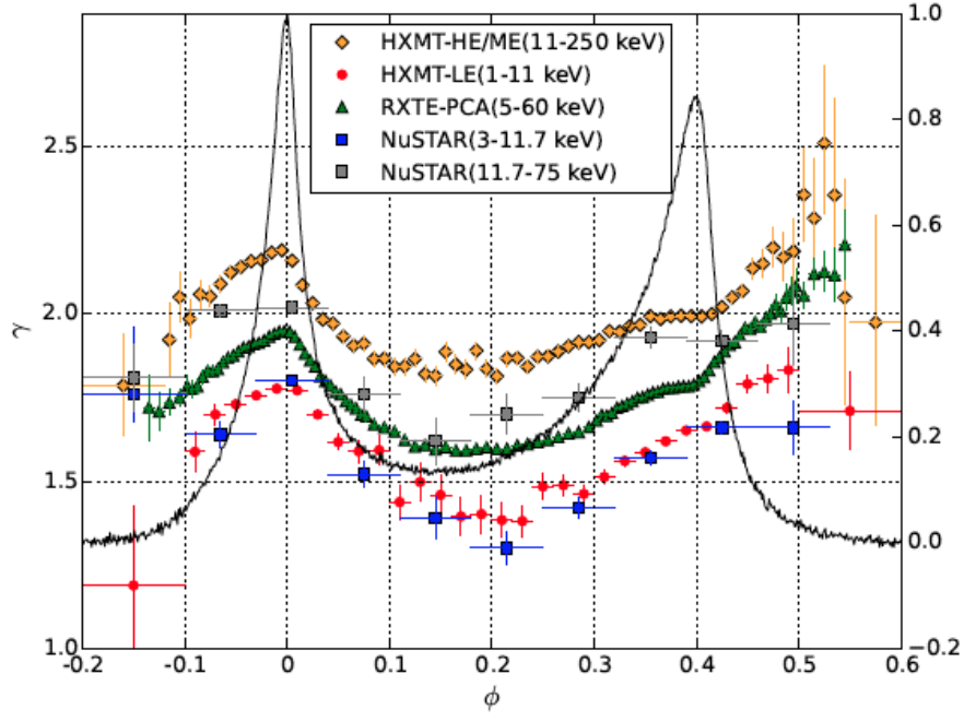
Fig.4-8 Phase-resolved spectra of the Crab pulsar (observed result of Insight-HXMT compared with that of RXTE/PCA and NuSTAR) (Tuo et al. 2019).
