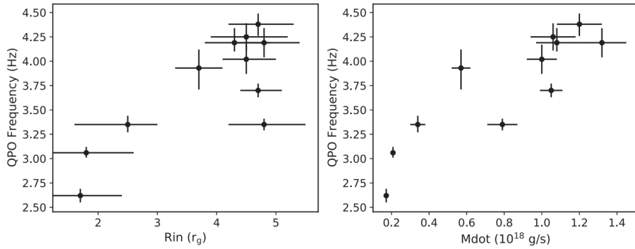
Fig 4-23 Left: correlation between the QPO frequency and inner disk radius; Right: correlation between the QPO frequency and mass accretion rate (H. Liu et al. 2021)
