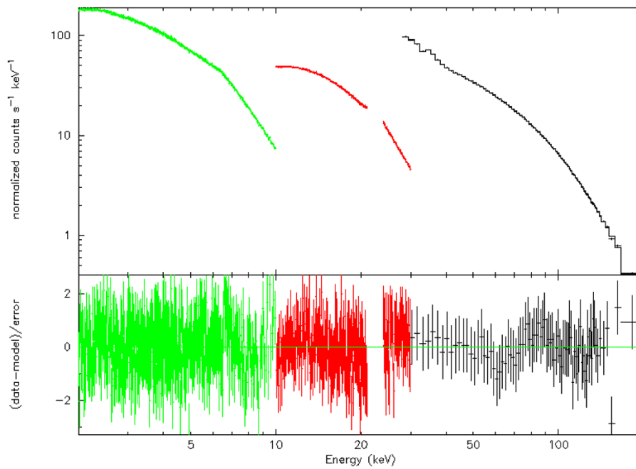
Fig. 4-32 Insight-HXMT spectra of MAXI J1820+070 in the intermediate state
