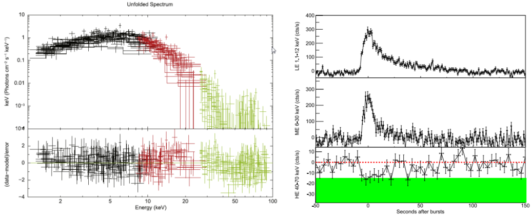
Fig. 4-38 Spectra and light curves of Type-I X-ray burst of 4U 1636–536 (Chen et al. 2018).
