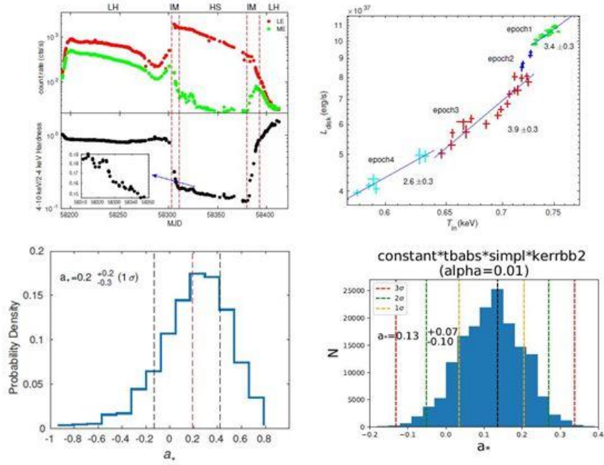
Fig. 4-20 Spin measurement of MAXI J1820+070 using the continuum fitting method (Guan et al. 2021; Zhao et al. 2021)
