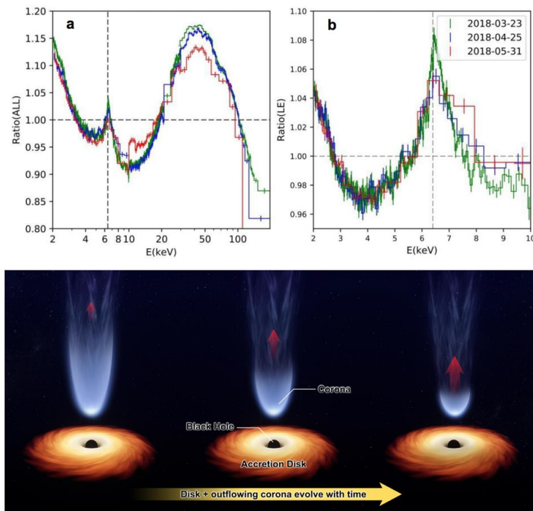
Fig.4-19 Acceleration of the outflowing coronal material when the corona contracts towards the black hole with decreasing height (You et al. 2021)
