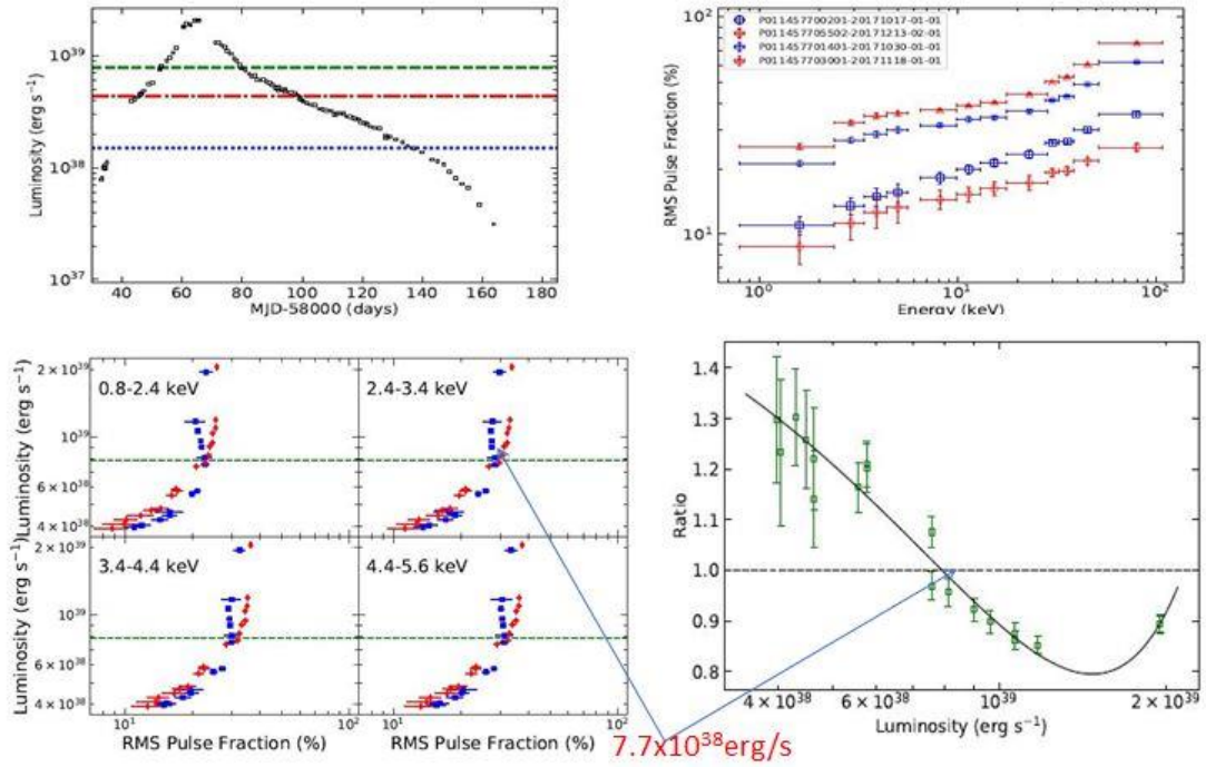
Fig.4-30 Pulse fraction evolution of Swift J0243.6+6124 monitored by Insight-HXMT (Wang et al. 2020)
