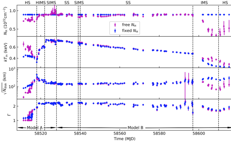
Fig 4-25 Peculiar behavior of MAXI J1346-630 in the hard state (Zhang et al. 2022)
